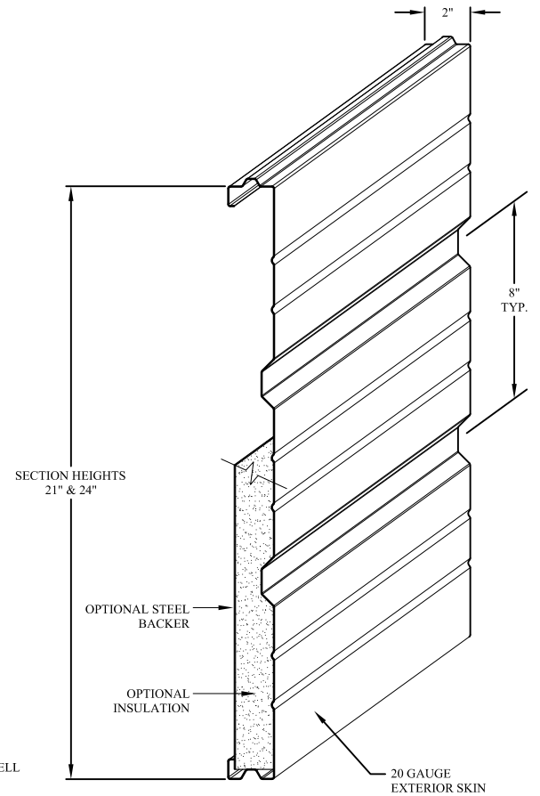
ISOMETRIC PROFILE
