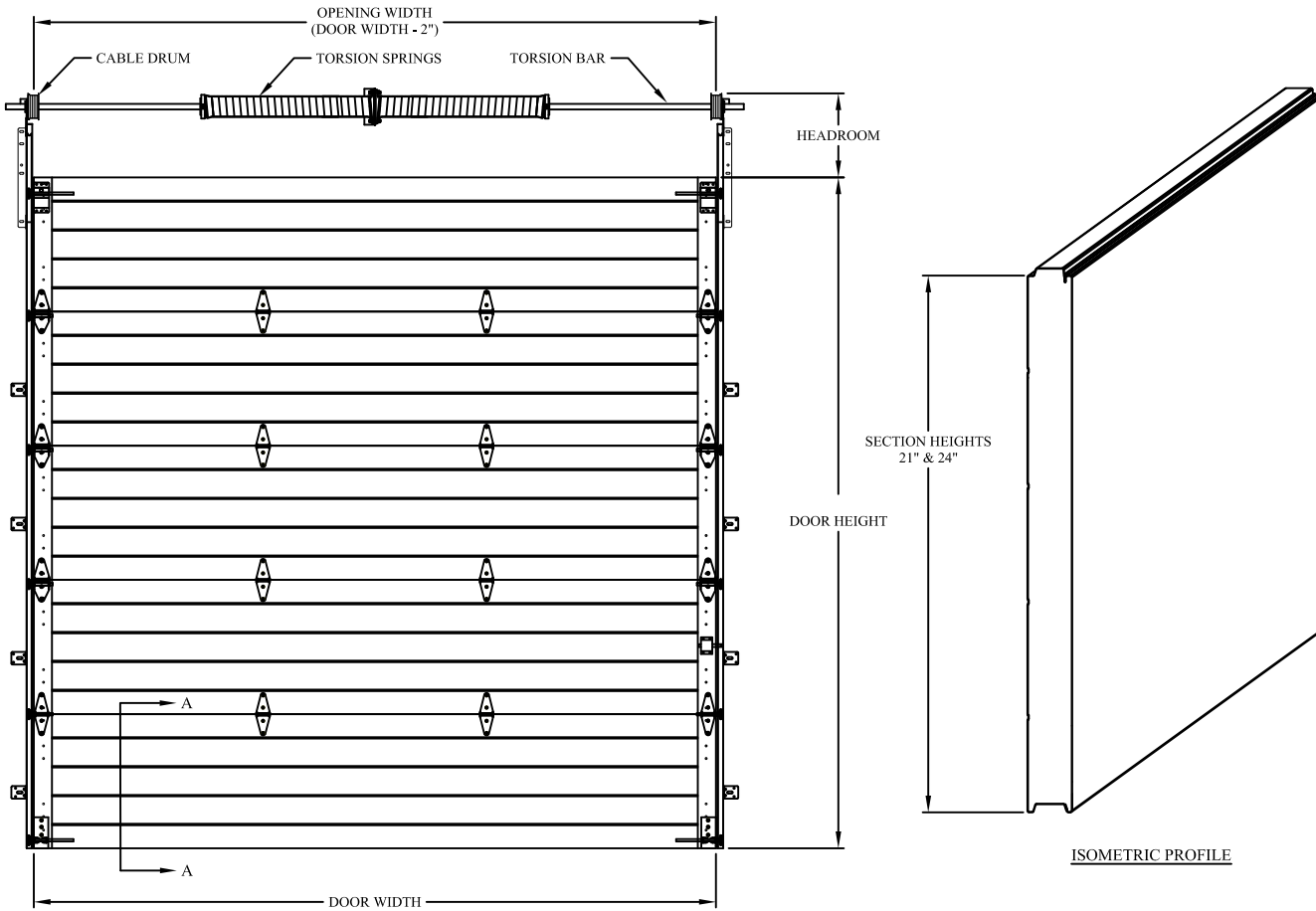
INTERIOR ELEVATION
