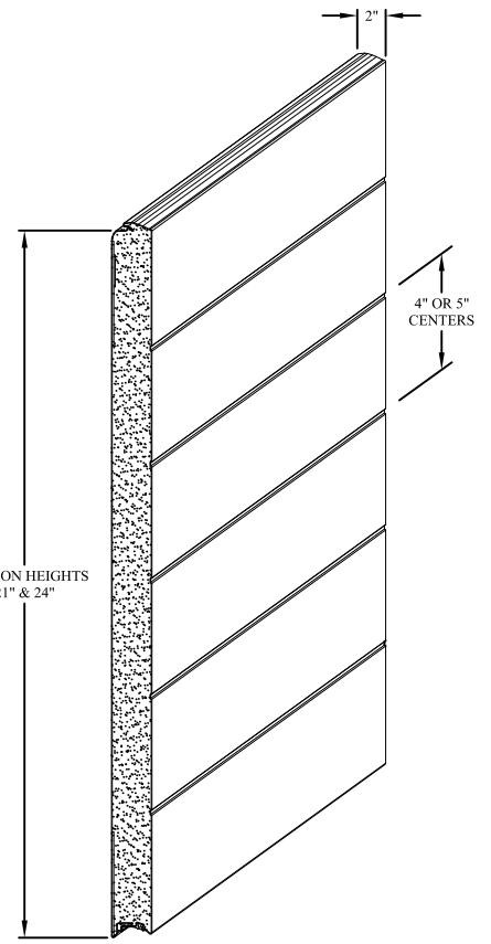
ISOMETRIC PROFILE
