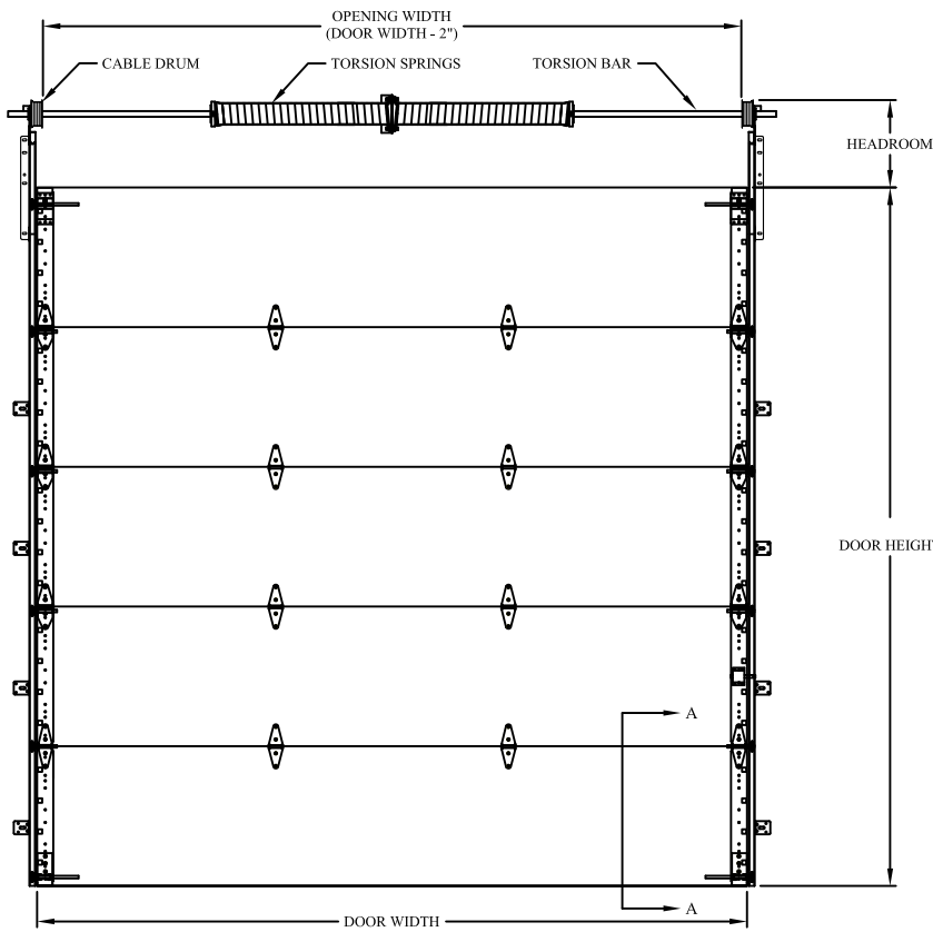
INTERIOR ELEVATION
