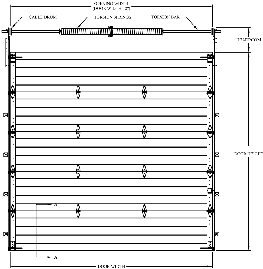
INTERIOR ELEVATION
