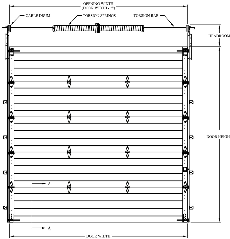
INTERIOR ELEVATION
