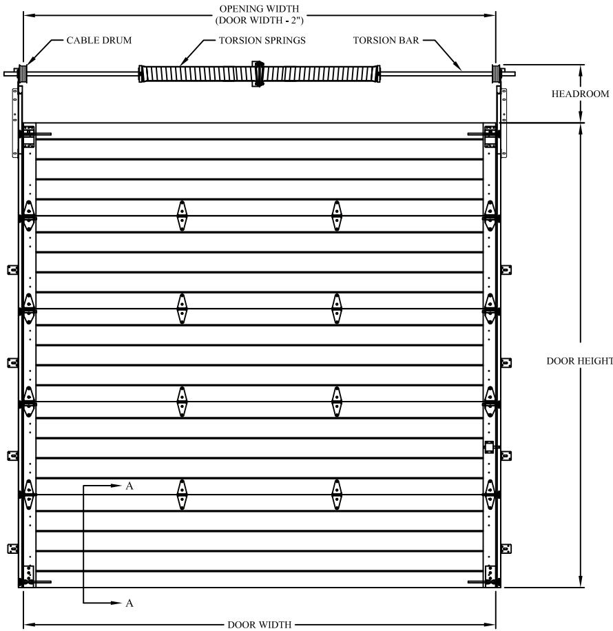
INTERIOR ELEVATION
