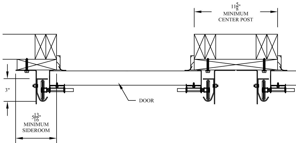
COMMERCIAL TAPERED REVERSE ANGLE MOUNT (LEG OUT) TO WOOD JAMB DETAIL
