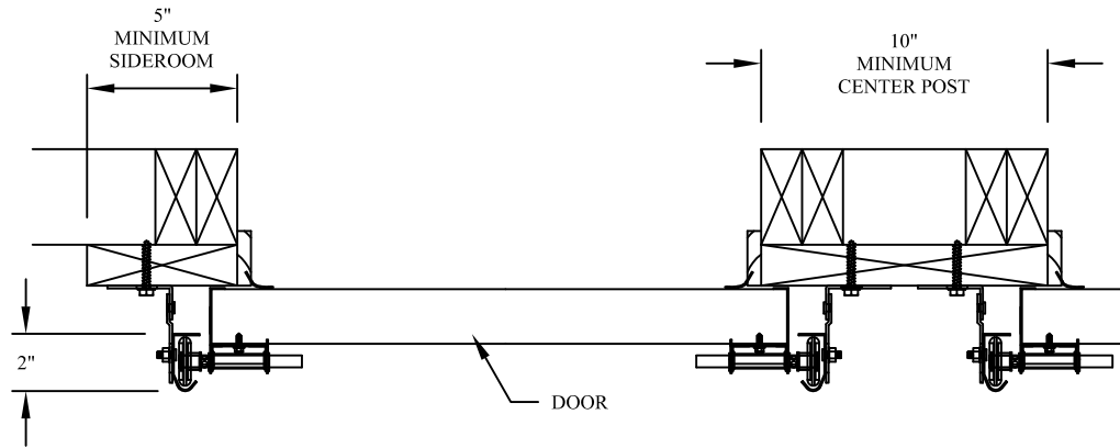
COMMERCIAL BRACKET MOUNT TO WOOD JAMB DETAIL
