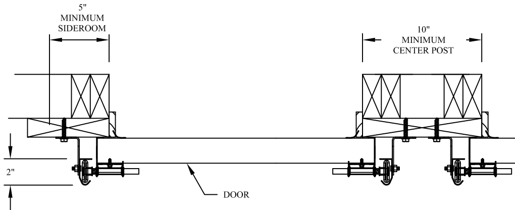
COMMERCIAL BRACKET MOUNT TO WOOD JAMB DETAIL
