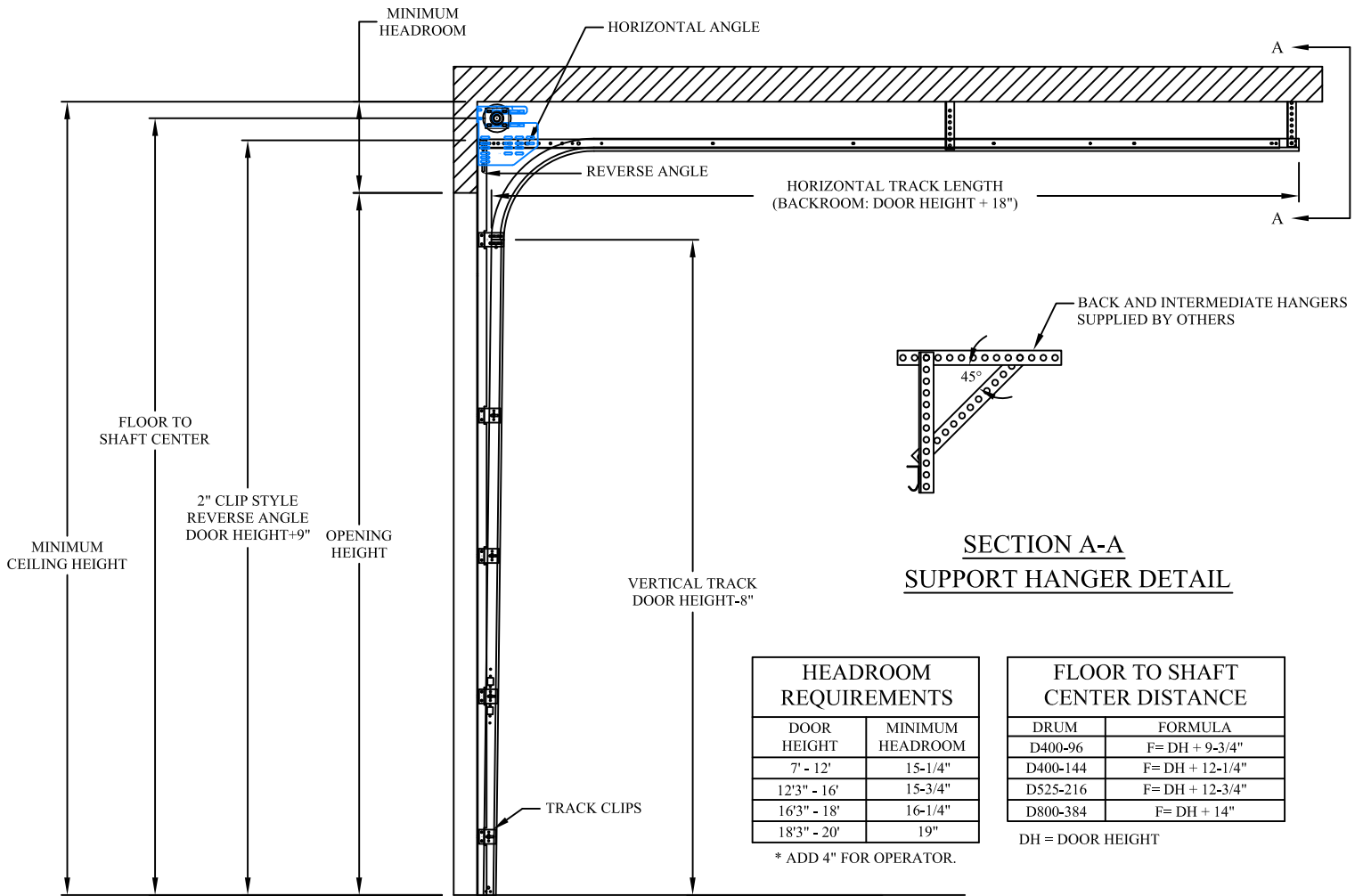
STANDARD LIFT ANGLE MOUNT TRACK SET DETAIL
